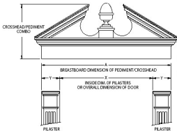
ONE PIECE CROSSHEAD AND PEDIMENT
