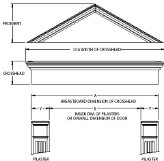
SEPARATE CROSSHEAD AND PEDIMENT
