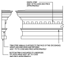
CROSSHEAD WITH DENTIL STRIP, TRIM STRIP AND BOTTOM TRIM
